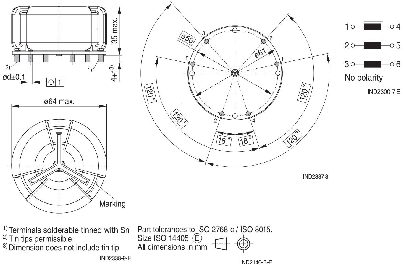
Figure 16 - B82747S4253A040, B82747S4303A041
