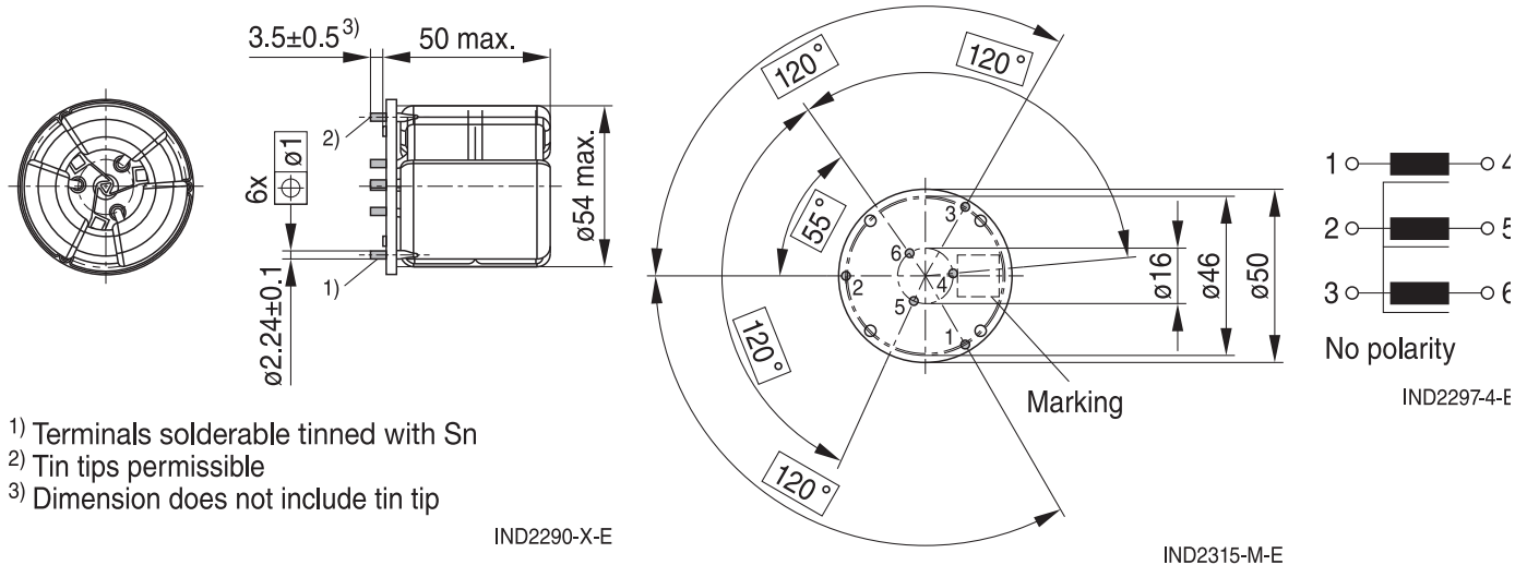
Figure 4 - B82746S4233A040
