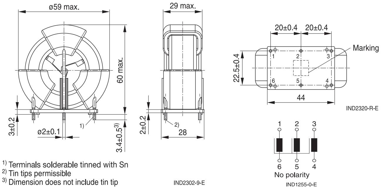
Figure 9 - B82747S4203A020
