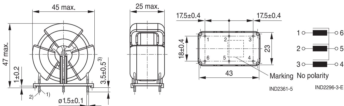
Figure 19 - B82746S4123N030
