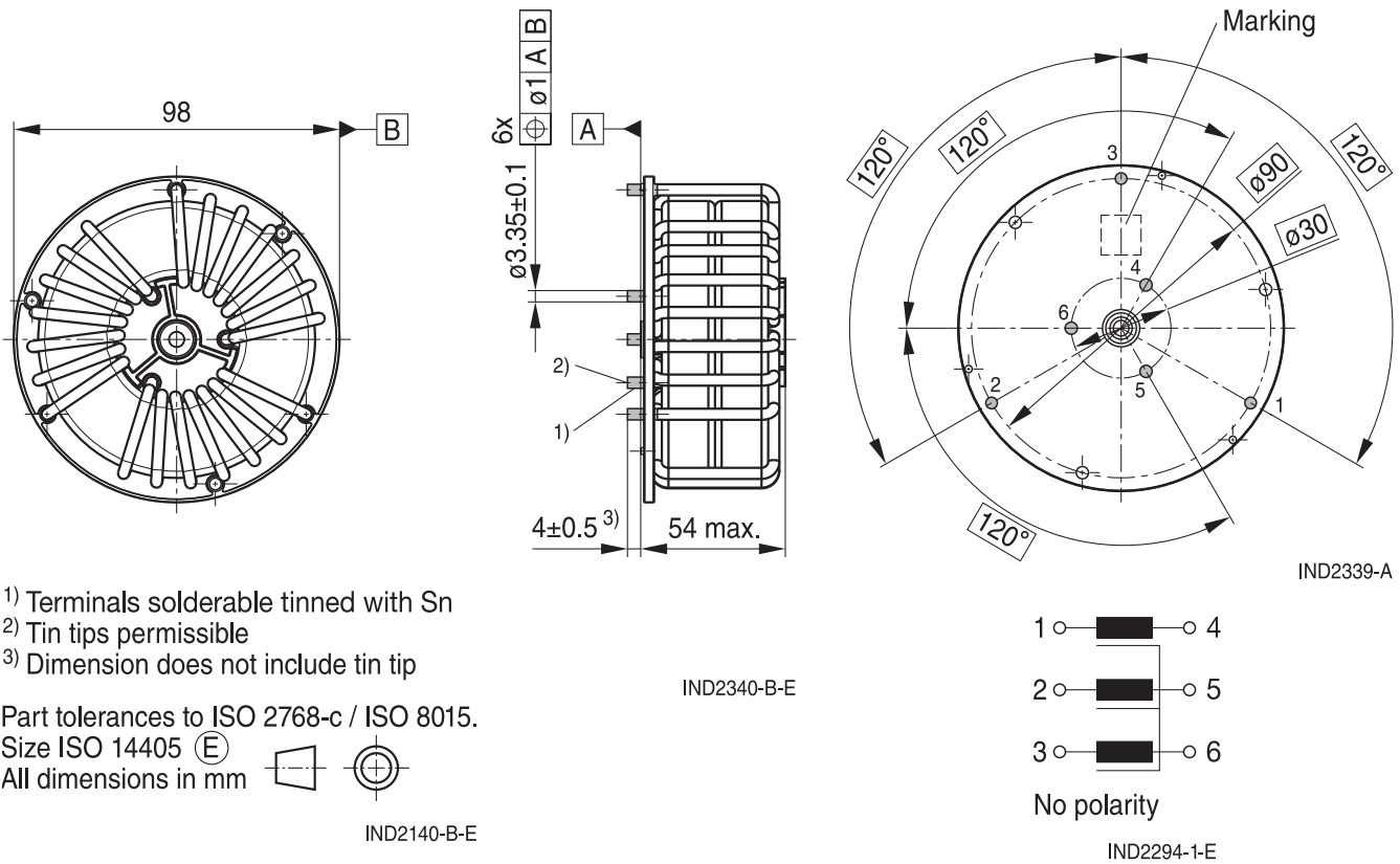
Figure 17 - B82748S6623N030
