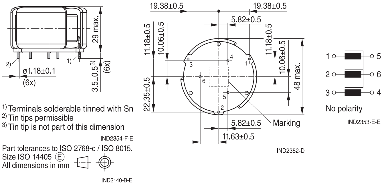
Figure 18 - B82746S4692A040
