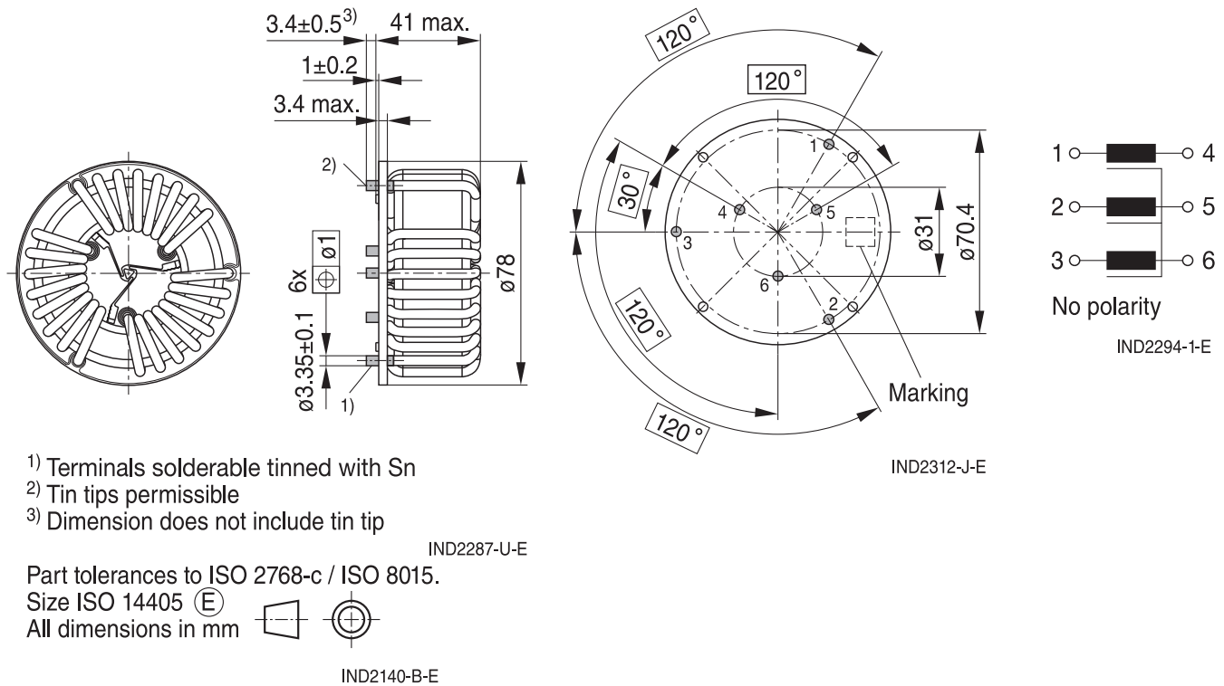
Figure 1 - B82748S4503A020
