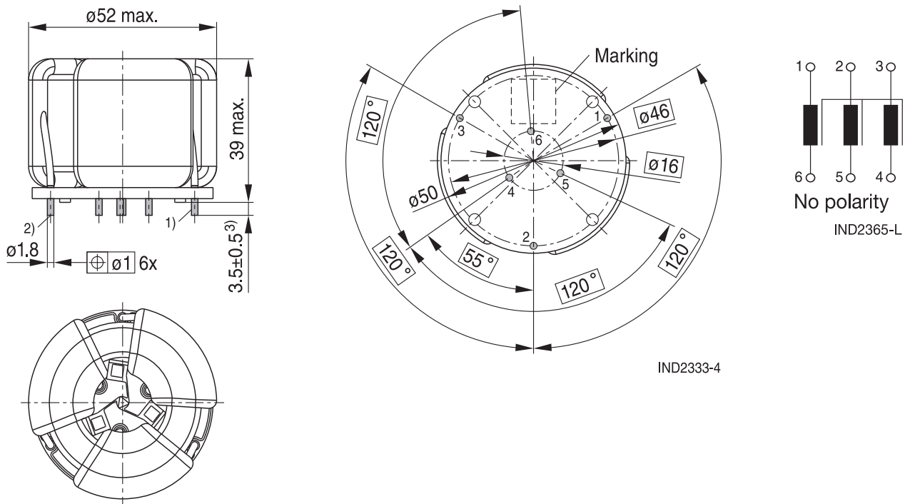
Figure 13 - B82746S4143A040
