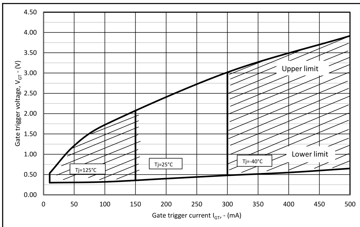
Fig.12 Gate characteristics
