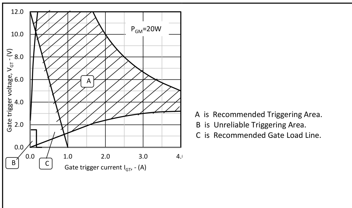
Fig.13 Gate characteristics
