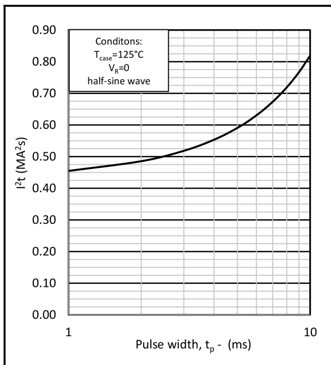
Fig.9 Single-cycle I^2t
