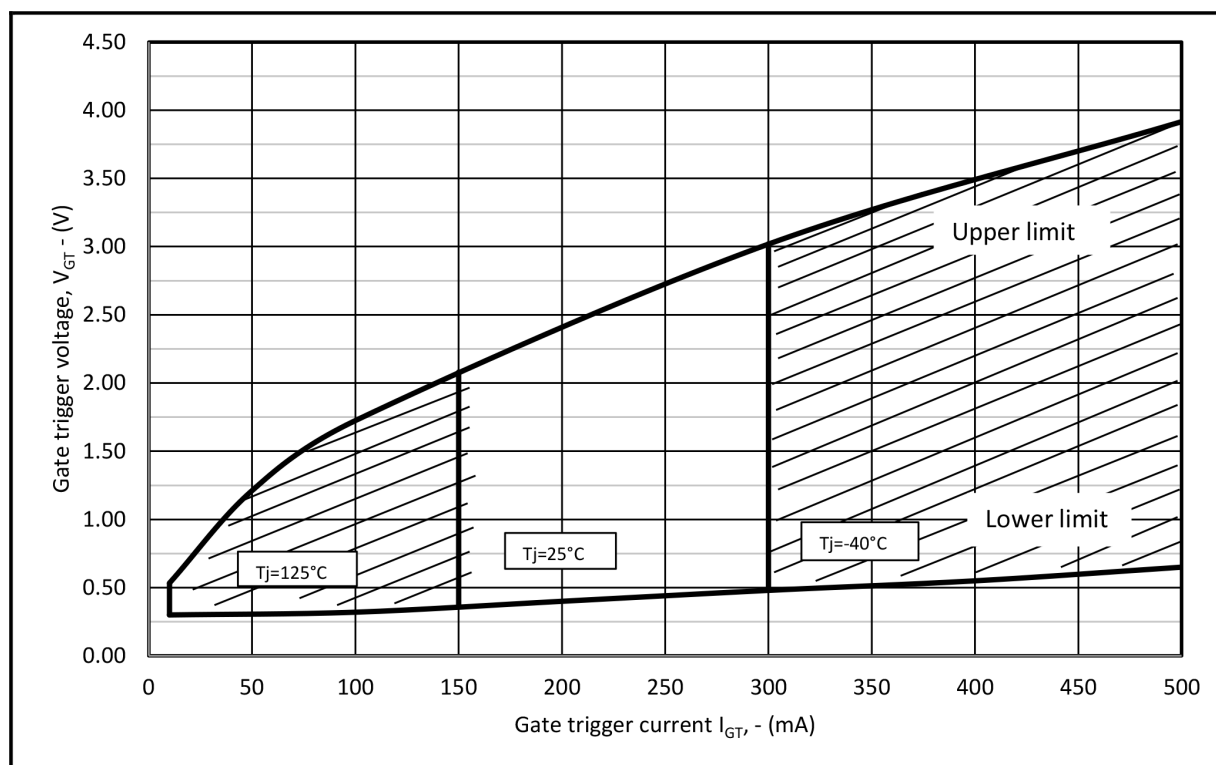
Fig.12 Gate characteristics
