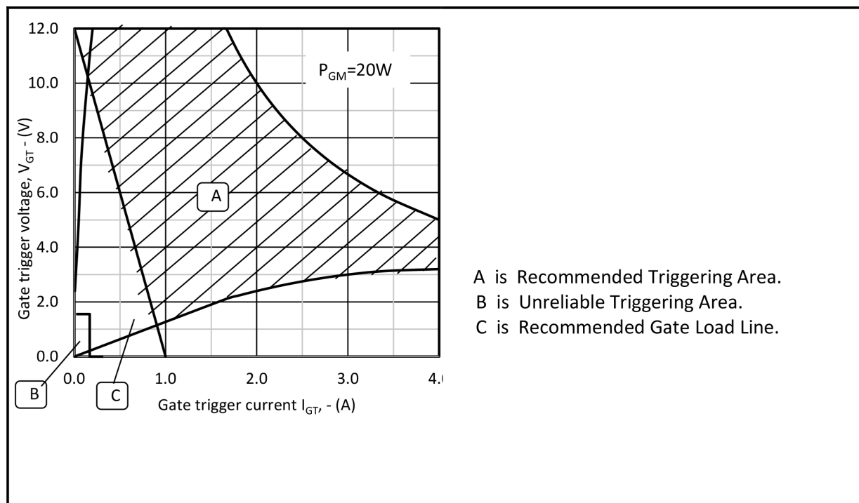
Fig.13 Gate characteristics
