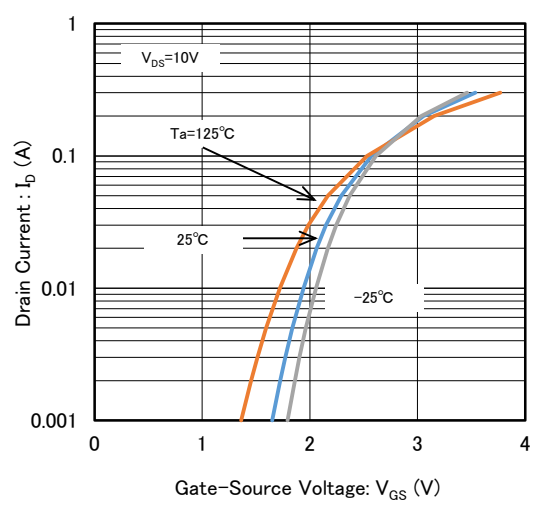
(2) Drain Current vs. Gate-Source Voltage
