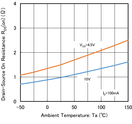
(4) Drain-Source On Resistance vs. Ambient Temperature
