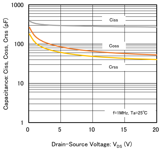
(7) Ciss, Coss, Crss vs. Drain-Source Voltage
