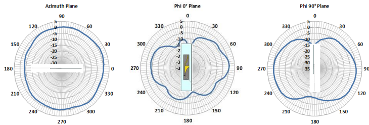
3700 MHz
