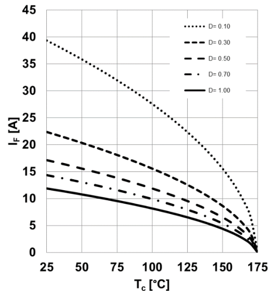
Figure 2. Diode forward current as function of temperature, parameter: T_{vj} \leq 175^\circ\text{C} , R_{\text{th(j-c)}}, \text{max} , D =duty cycle, V_{\text{th}} , R_{\text{diff}} @ T_{vj}=175^\circ\text{C}
