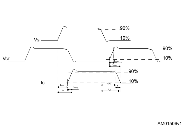
Figure 29. Switching waveform
