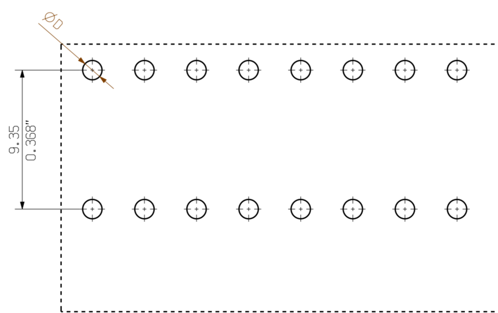
HOLE PATTERN
