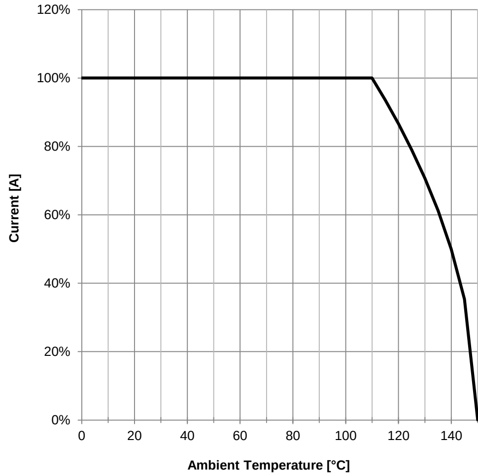
Derating Curve:
