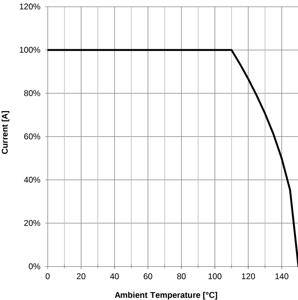
Derating Curve:
