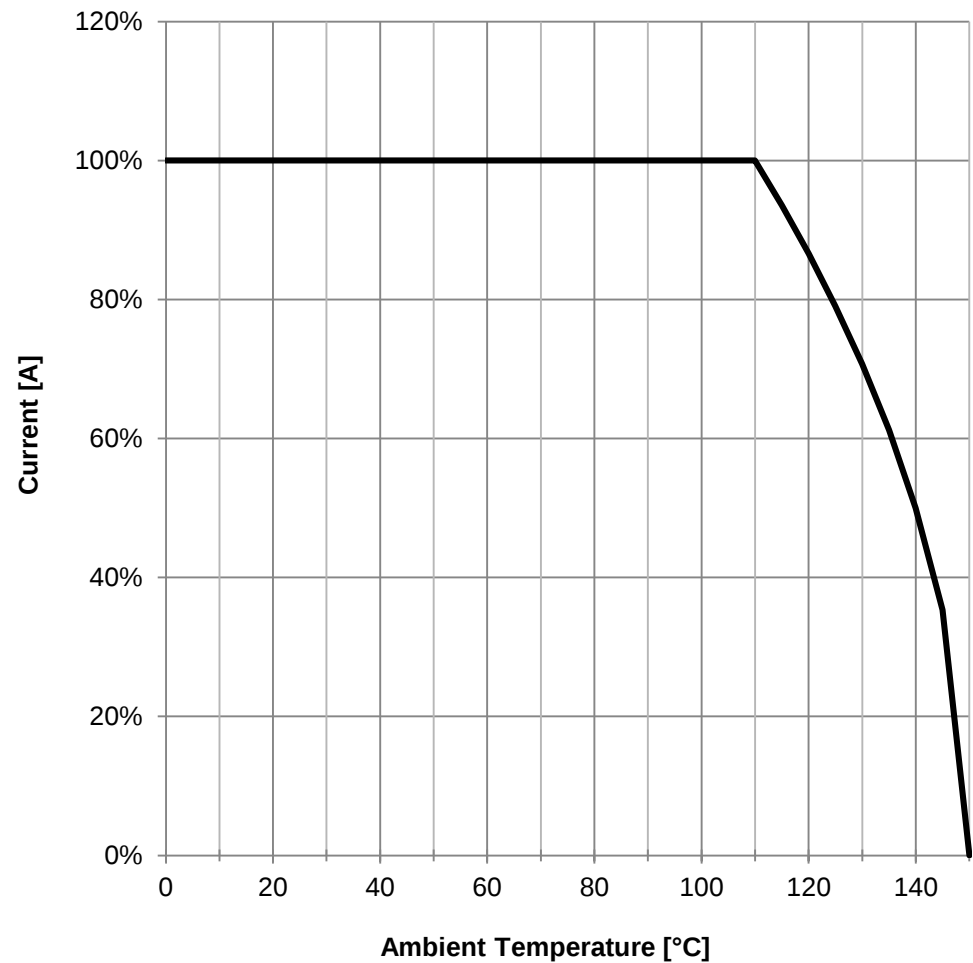
Derating Curve:
