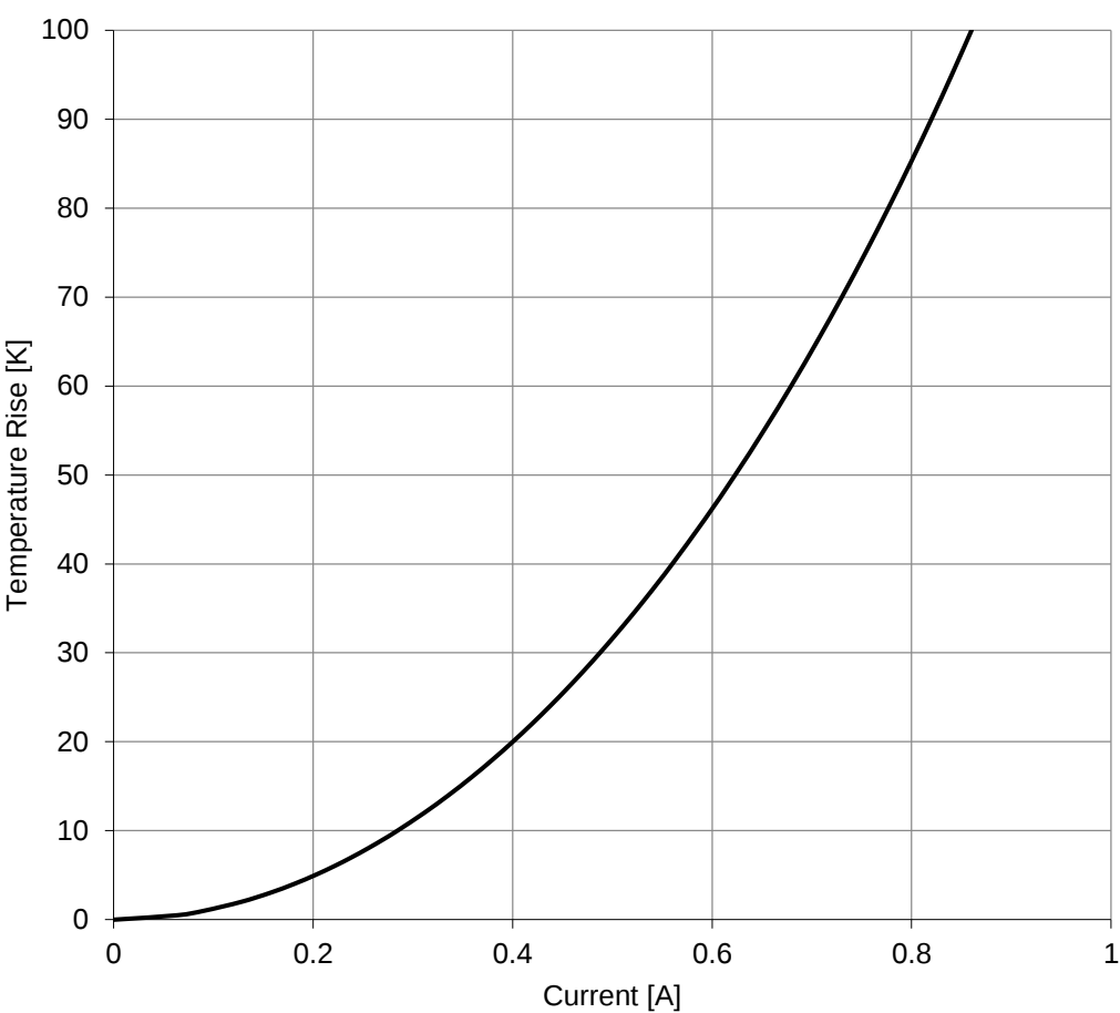
Typical Temperature Rise vs. Current Characteristics:
