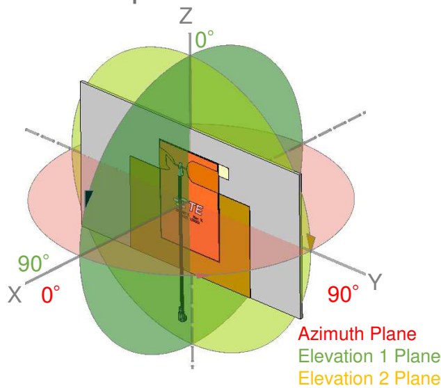
Test setup
