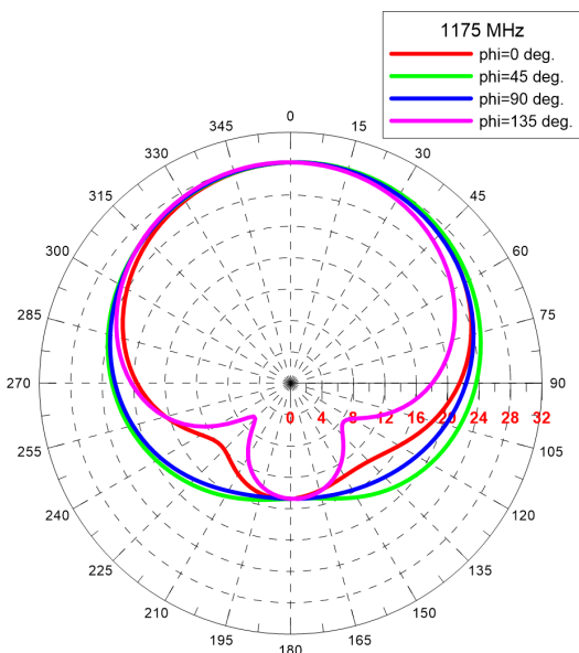
RHCP Realized Gain [dBic] - Elevation Cuts
