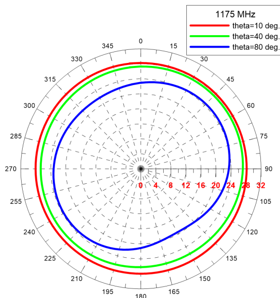
RHCP Realized Gain [dBic] - Azimuth Cuts
