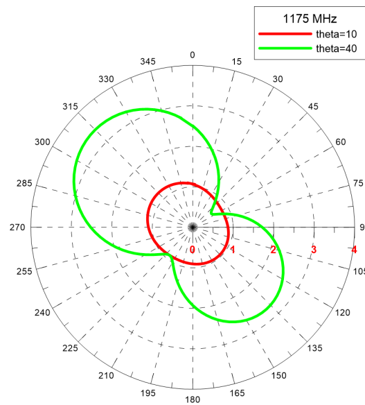
Axial Ratio [dB] - Azimuth Cuts
