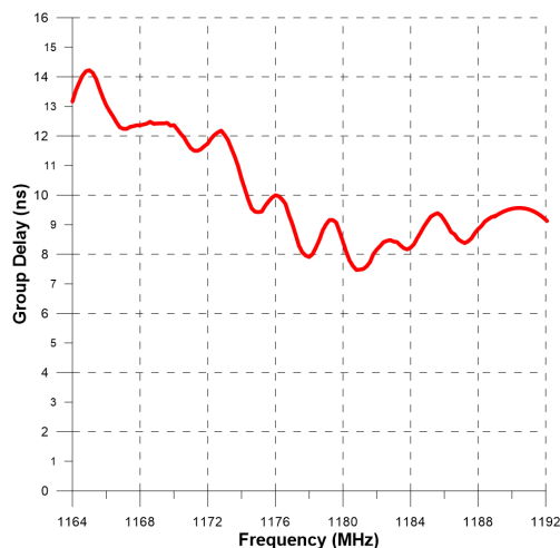
< 2 ns group delay variation over L5-band.
