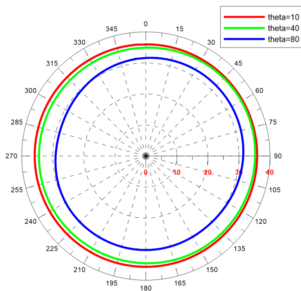
RHCP Realized Gain [dBic] - Azimuth Cuts
