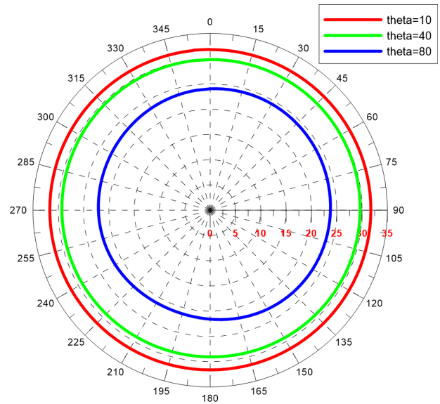
RHCP Realized Gain [dBi] - Azimuth Cuts
