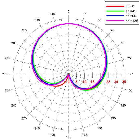
RHCP Realized Gain [dBi] - Elevation Cuts
