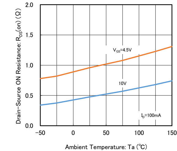
(4) Drain-Source On Resistance vs. Ambient Temperature
