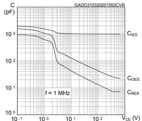
Figure 12. Capacitance variations
