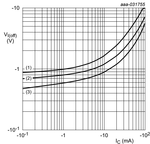
Fig. 36. NHUMD9, TR2 (PNP): Off-state input voltage as a function of collector current; typical values
