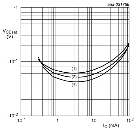
Fig. 37. NHUMD9, TR2 (PNP): Collector-emitter saturation voltage as a function of collector current; typical values
