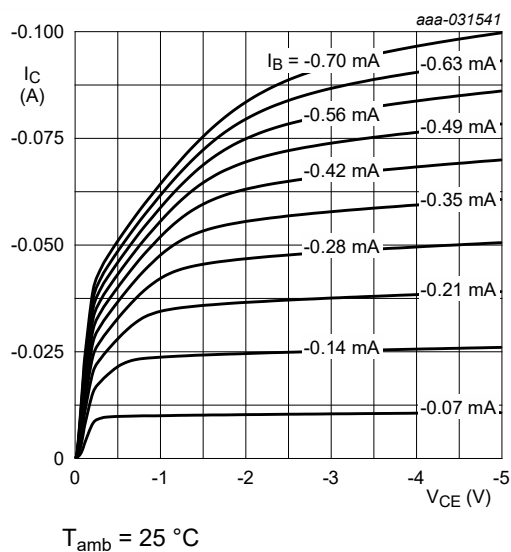
Fig. 10. NHUMB11: Collector current as a function of collector-emitter voltage; typical values
