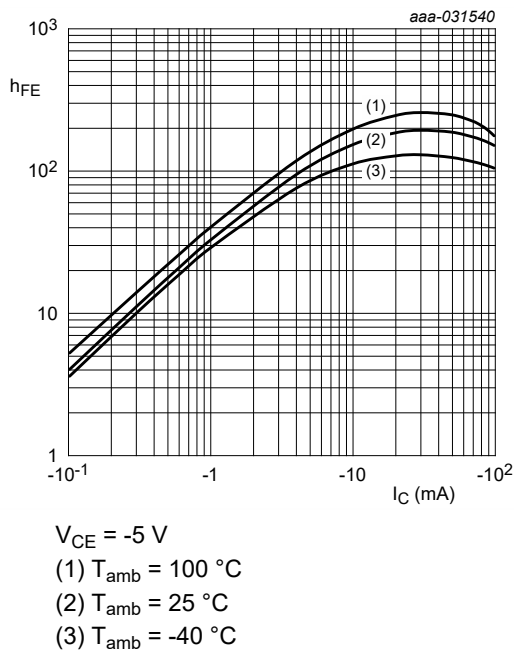
Fig. 9. NHUMB11: DC current gain as a function of collector current; typical values
