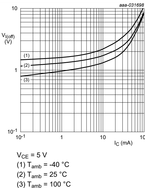
Fig. 7. NHDTC114ET: Off-state input voltage as a function of collector current; typical values
