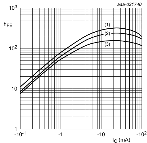
V_{CE} = -5 V (1) T_{amb} = 100 °C (2) T_{amb} = 25 °C (3) T_{amb} = -40 °C
