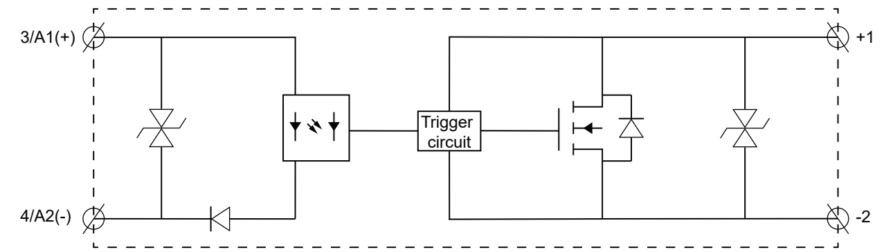
Fig. 10 RM1D functional diagram
