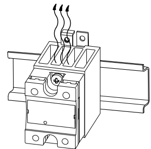
Fig. 14 Mount heatsink with fins in the vertical orientation to guarantee the best possible airflow through the heatsink.
