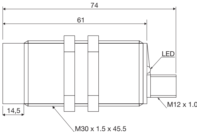
Fig. 9 Plug CA30CAN...M1IO
