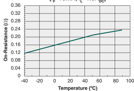
Typical On-Resistance vs. Temperature ( I_F=10\text{mA} , I_L=1.0\text{A}_{DC} )
