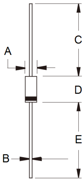
DO-204AC (DO-15)
