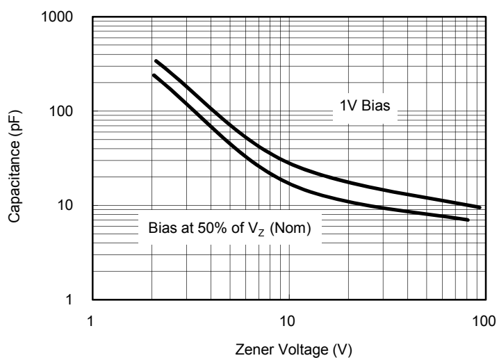
Fig. 5 Typical Capacitance
