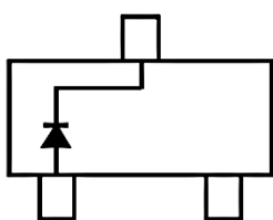
BAT54
