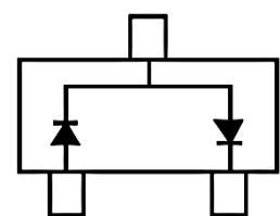
BAT54S
