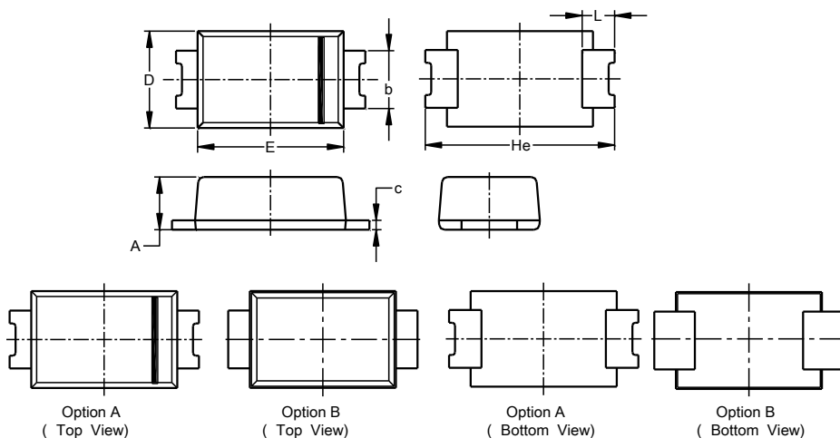
SOD123F (Standard)
