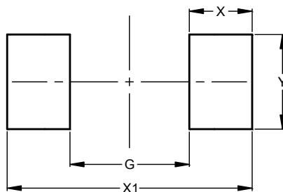
SOD123F (Standard)
