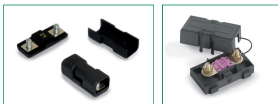
MIDI inline fuseholder (Left) MIDI covered fuseholder (Right)
