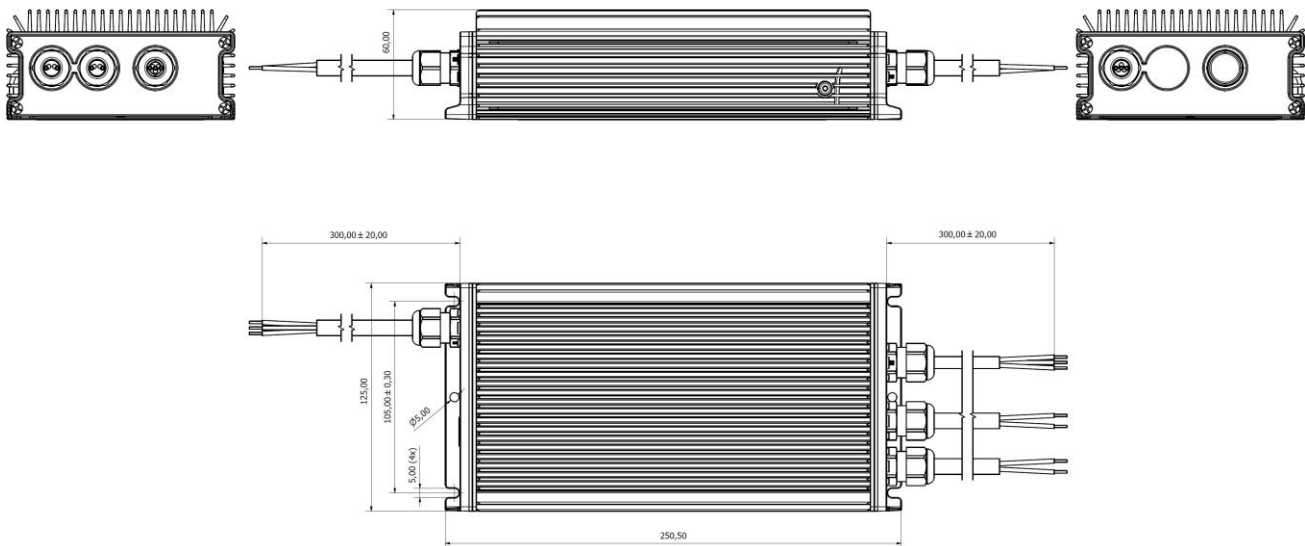
Figure 3. Mechanical drawing
