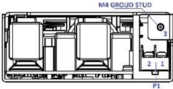
Figure 3. Front View - ACC750-1T24 / ACC750-1T48 Models
