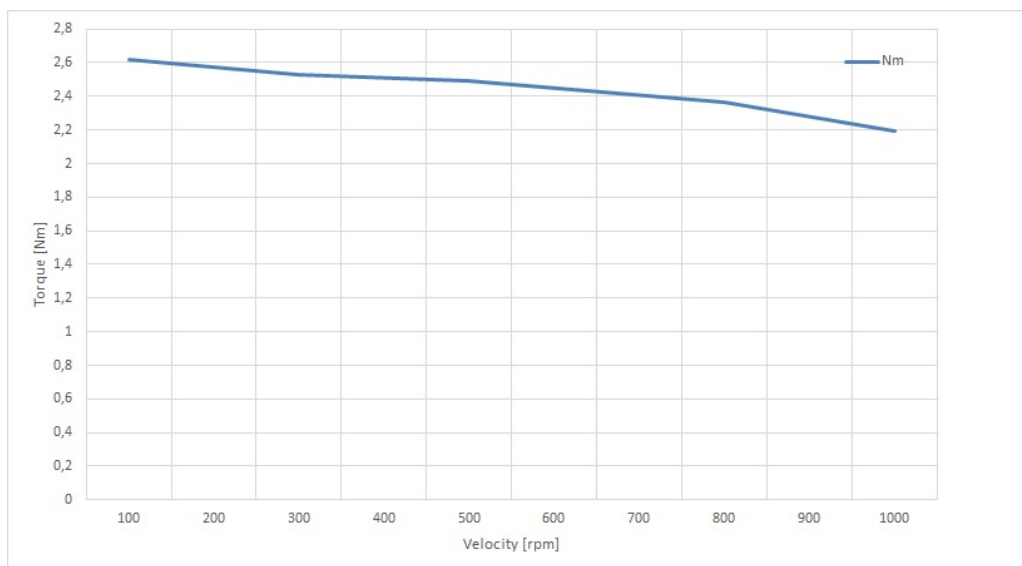
Figure 7: PD60-4H-1278 torque vs. velocity 48V / 9A, 256 \mu steps
