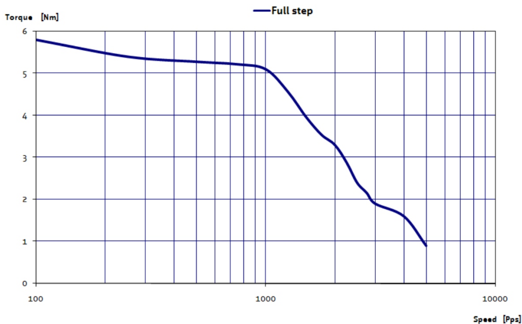
Figure 8: PD86-3-1278 torque vs. velocity 48V / 5.5A, 256 \mu steps
