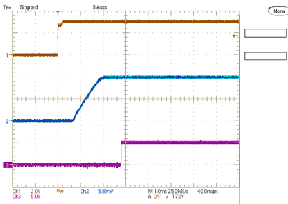
On/Off Enable Delay (Vin=12.0V, Vout=1.0V, Iout=12A, Clad=660uF) Trace1=Enable, Trace2=Vout. Trace3=P.G
