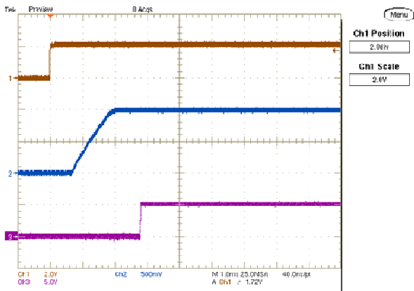
On/Off Enable Delay (Vin=5.0V, Vout=1.0V, Iout=12A, Load=660uF) Trace1=Enable, Trace2=Vout, Trace3=P.G
