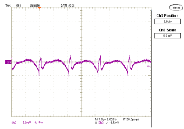
Output Ripple and Noise (Vin=5.0V, Vout=0.7V, Iout=12A, Load=660uF, ScopeBW=20MHz)
