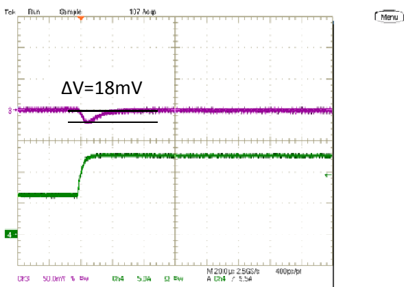
Step Load Transient Response (Vin=5.0V, Vout=1.0V, Load=660uF, Iout=6A to 12A, 1.2A/us) Trace 3=Vout, 50 mV/div, Trace 4=Iout, 5A/div.
