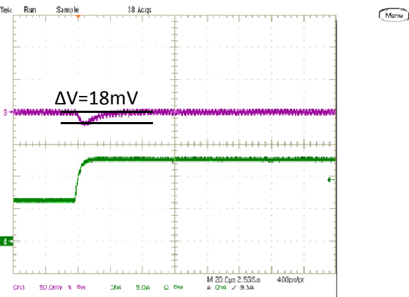
Step Load Transient Response (Vin=5.0V, Vout=1.8V, Load=660uF, Iout=6A to 12A, 1.2A/us) Trace 3=Vout, 50 mV/div, Trace 4=Iout, 5A/div.
