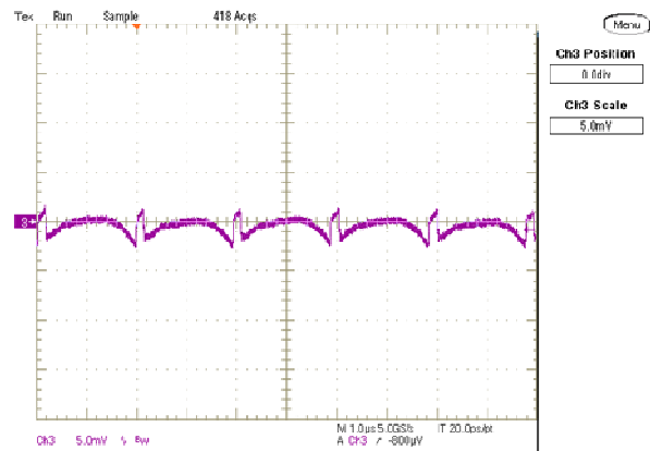
Output Ripple and Noise (Vin=5.0V, Vout=1.0V, Iout=12A, Load=660uF, ScopeBW=20MHz)
