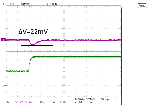
Step Load Transient Response (Vin=12.0V, Vout=1.0V, Clad=660uF, Iout=6A to 12A, 1.2A/us) Trace 3=Vout, 50 mV/div, Trace 4=Iout, 5A/div.
