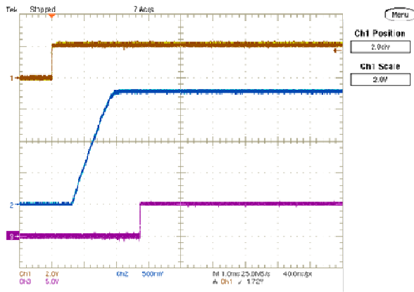
On/Off Enable Delay (Vin=5.0V, Vout=1.8V, Iout=12A, Load=660uF) Trace1=Enable, Trace2=Vout, Trace3=P.G
