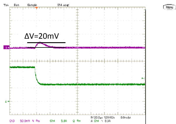
Step Load Transient Response (Vin=12.0V, Vout=1.0V, Clad=660uF, Iout=12A to 6A, 1.2A/us) Trace 3=Vout, 50 mV/div, Trace 4=Iout, 5A/div.
