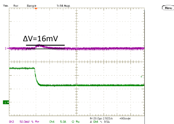
Step Load Transient Response (Vin=5.0V, Vout=1.8V, Load=660uF, Iout=12A to 6A, 1.2A/us) Trace 3=Vout, 50 mV/div, Trace 4=Iout, 5A/div.
