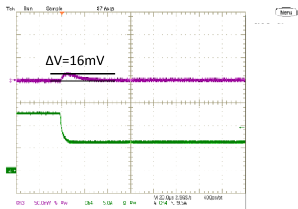
Step Load Transient Response (Vin=5.0V, Vout=1.0V, Load=660uF, Iout=12A to 6A, 1.2A/us) Trace 3=Vout, 50 mV/div, Trace 4=Iout, 5A/div.
