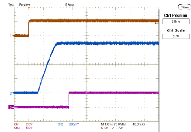
On/Off Enable Delay (Vin=5.0V, Vout=0.7V, Iout=12A, Load=660uF) Trace1=Enable, Trace2=Vout, Trace3=P.G
