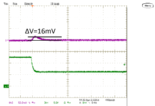
Step Load Transient Response (Vin=5.0V, Vout=0.7V, Load=660uF, Iout=12A to 6A, 1.2A/us) Trace 3=Vout, 50 mV/div, Trace 4=Iout, 5A/div.
