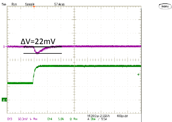
Step Load Transient Response (Vin=12.0V, Vout=1.8V, Cload=660uF, Iout=6A to 12A, 1.2A/us) Trace 3=Vout, 50 mV/div, Trace 4=Iout, 5A/div.
