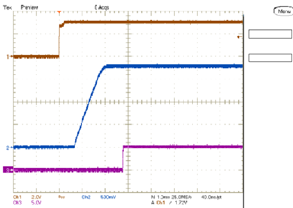
On/Off Enable Delay (Vin=12.0V, Vout=1.8V, Iout=12A, Cload=660uF) Trace1=Enable, Trace2=Vout, Trace3=P.G
