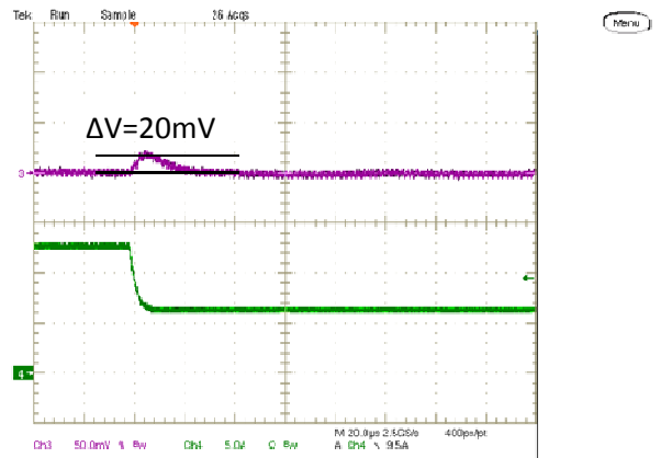
Step Load Transient Response (Vin=12.0V, Vout=1.8V, Cload=660uF, Iout=12A to 6A, 1.2A/us) Trace 3=Vout, 50 mV/div, Trace 4=Iout, 5A/div.
