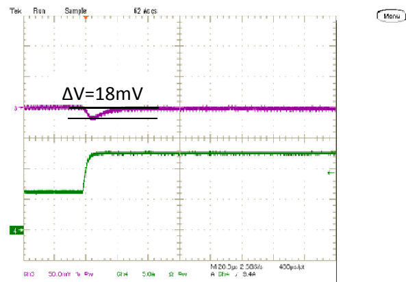
Step Load Transient Response (Vin=5.0V, Vout=0.7V, Load=660uF, Iout=6A to 12A, 1.2A/us) Trace 3=Vout, 50 mV/div, Trace 4=Iout, 5A/div.
