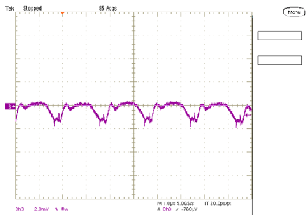
Output Ripple and Noise (Vin=12.0V, Vout=1.0V, Iout=12A, Clad=660uF, ScopeBW=20MHz)
