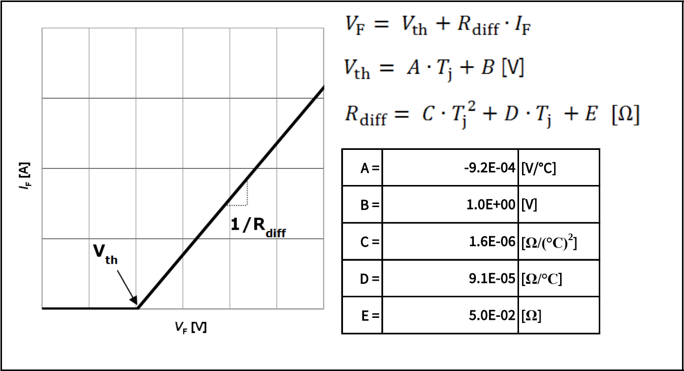
Figure 6 Simplified forward characteristics model V_F = f(I_F) ; -40^\circ\text{C} < T_j < 175^\circ\text{C} ; I_F < 16 A
