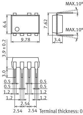
External dimensions
