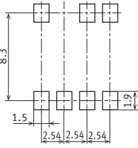
Recommended mounting pad (TOP VIEW)
