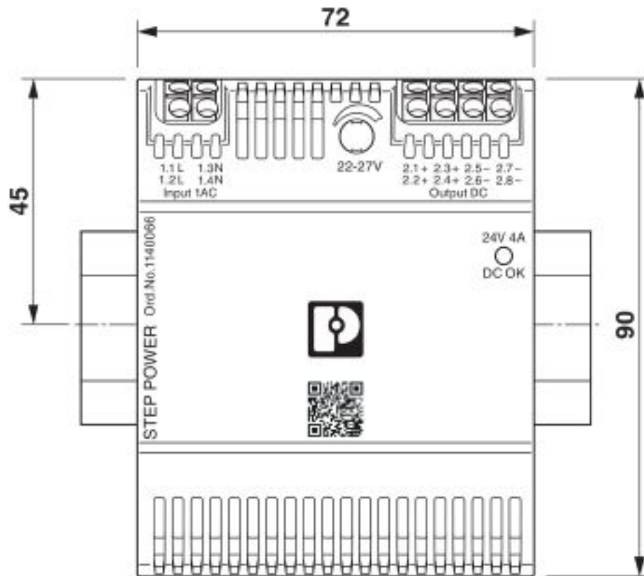
Dimensional drawing
