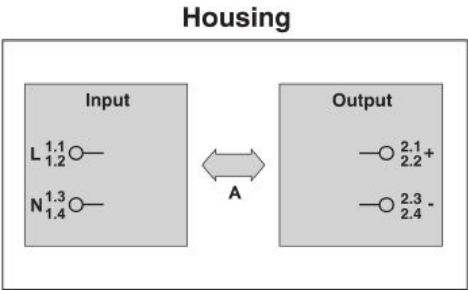
Schematic diagram
