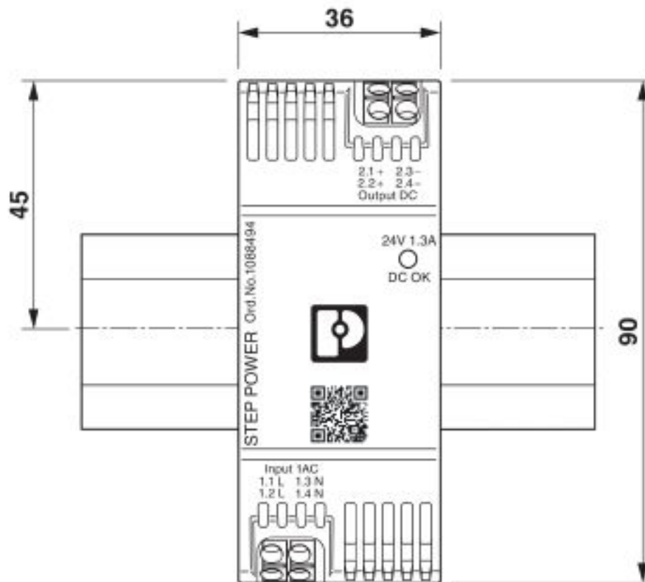
Dimensional drawing
