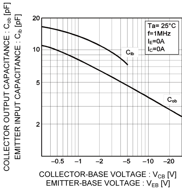
Fig.9 Collector Output Capacitance vs. ollector-Base Voltage Emitter Input Capacitance vs. Emitter-Base Voltage
