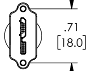
USB 3.0 SERIES MICRO-B PLUG MOLDED, BLACK
