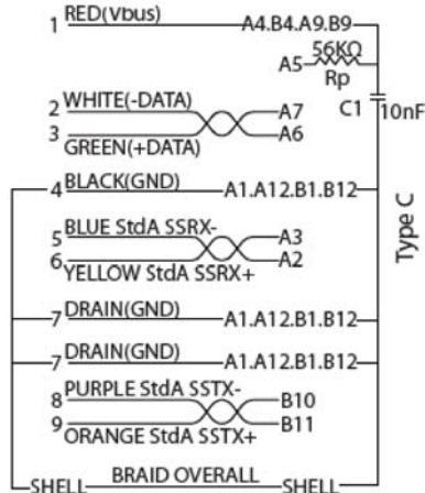
"P1" WIRING MAP "P2"
