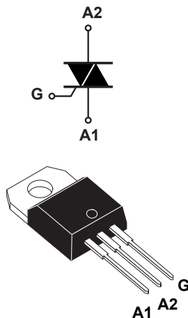
TO-220AB insulated
