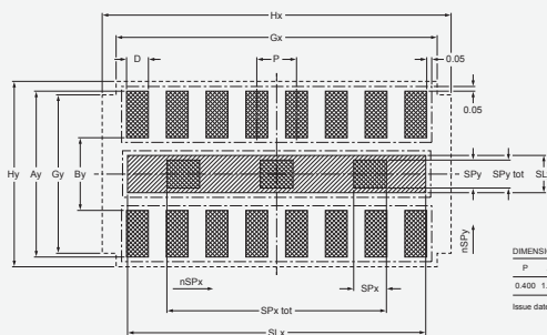
DFN3314-16 (SOT974-2)
