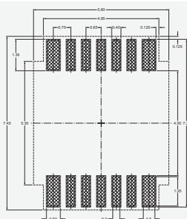
TSSOP14 (SOT402-1)
