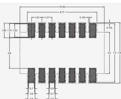
SO14 (SOT108-1)
