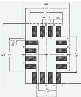
XQFN16 (SOT1161-1)
