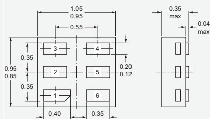
XSON6 (SOT1115)
