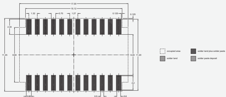
SO24 (SOT137-1)
