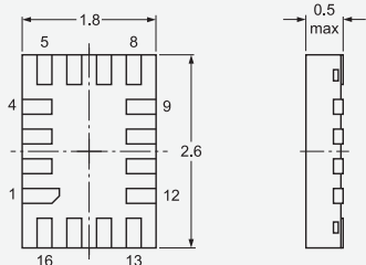
XQFN16 (SOT1161-1)
