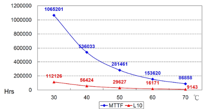
MTTF & L10 Curve
