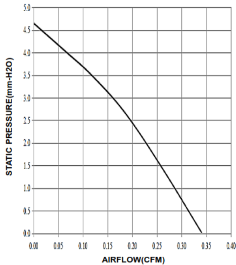
Fan Performance Curve
