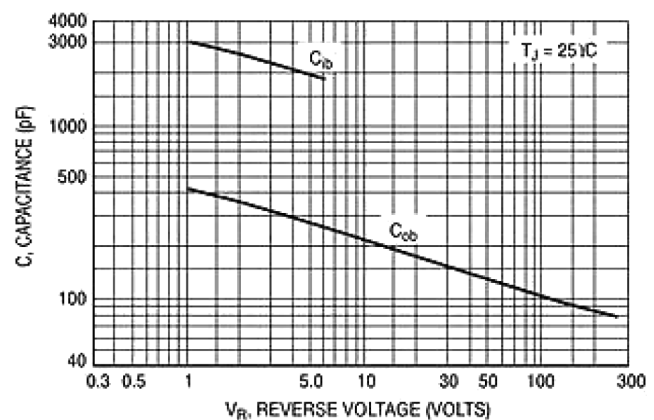
Figure 2. Capacitances
