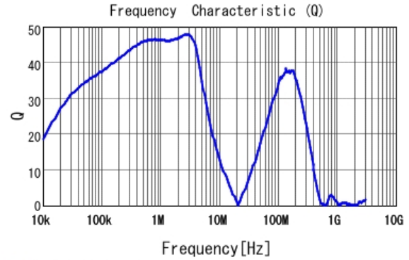
■ 1217AS-H-150M Q
