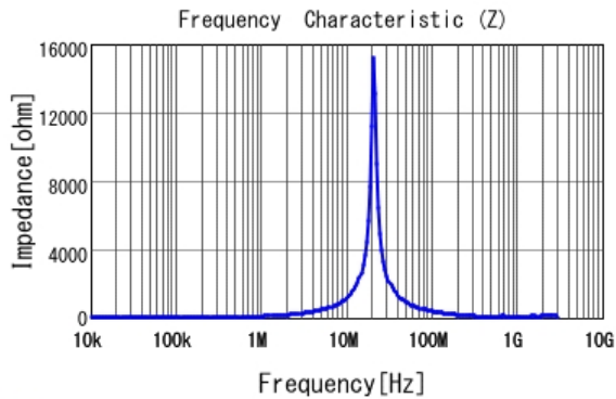
■ 1217AS-H-150M |Z|
