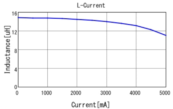
■ 1217AS-H-150M L-Current 20degC
