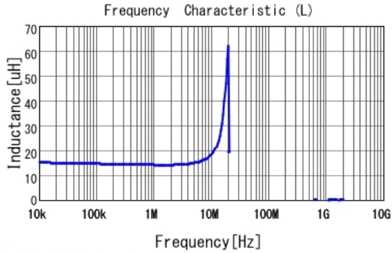
■ 1217AS-H-150M L
